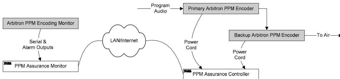
Figure 3. In-series PPM Assurance installation.
